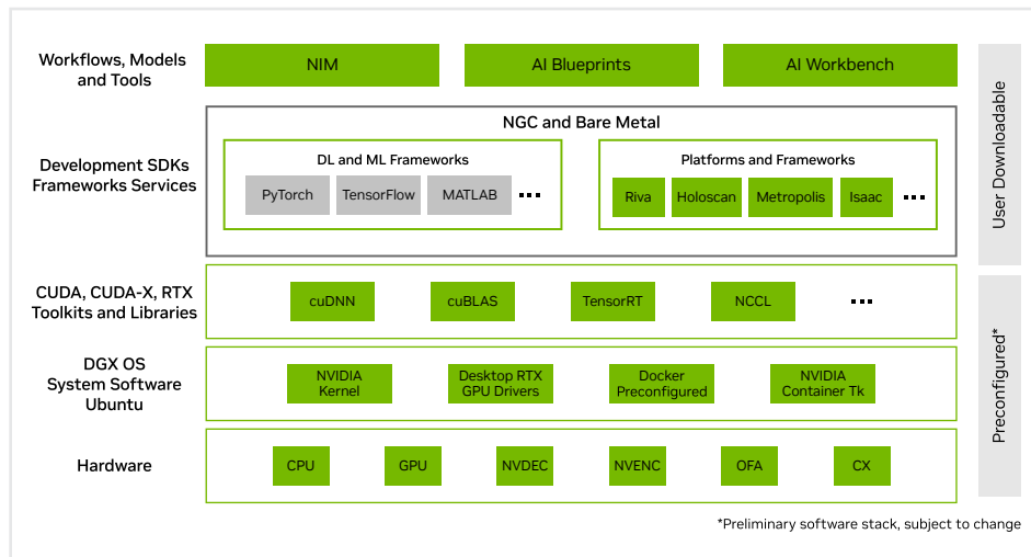
NVIDIA DGX Spark software stack
